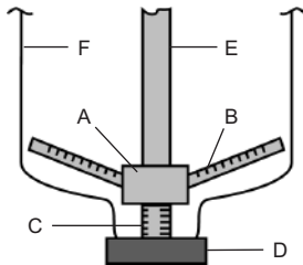
Z-style distributor shown mounted on blind flange.
